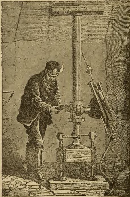
Fig. 48. ROCK DRILLING WITH COMPRESSED-AIR.
